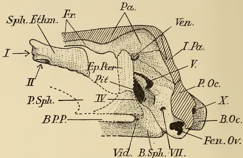
FIG. 5.— Scymnognathus whaitsi . B.M.N.H., R4053. Lateral view of the left side of the brain-case, modified after Watson. \times \frac{2}{3} .
